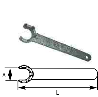
ER-M-Spanner
